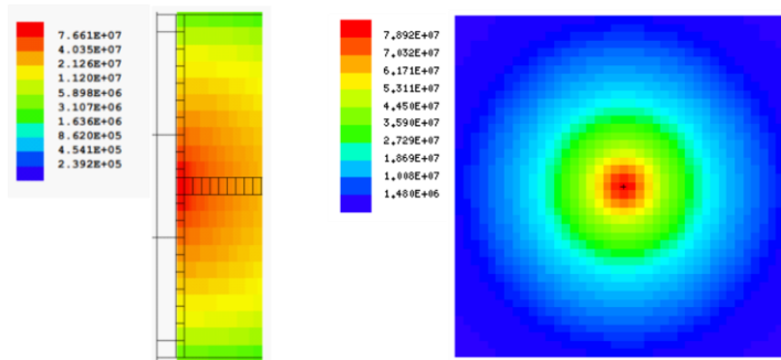
Fig. 3: MCNP results about the 2D neutron flux spatial distribution in depth (left) and along superficial tissues (right) obtained by a 6 cm window diameter.
